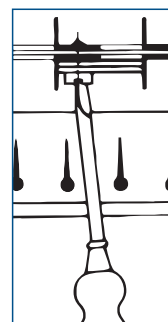
Pormenor 4
